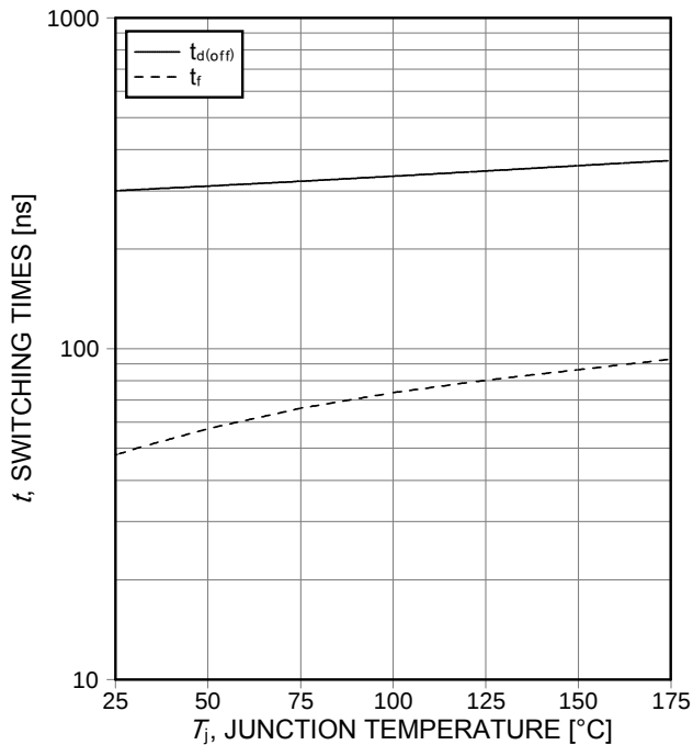
Figure 11. Typical switching times as a function of junction temperature (ind. load, V_{CE}=600\text{V} , V_{GE}=15/0\text{V} , I_C=15\text{A} , R_G=14,6\Omega , test circuit in Fig. E)
